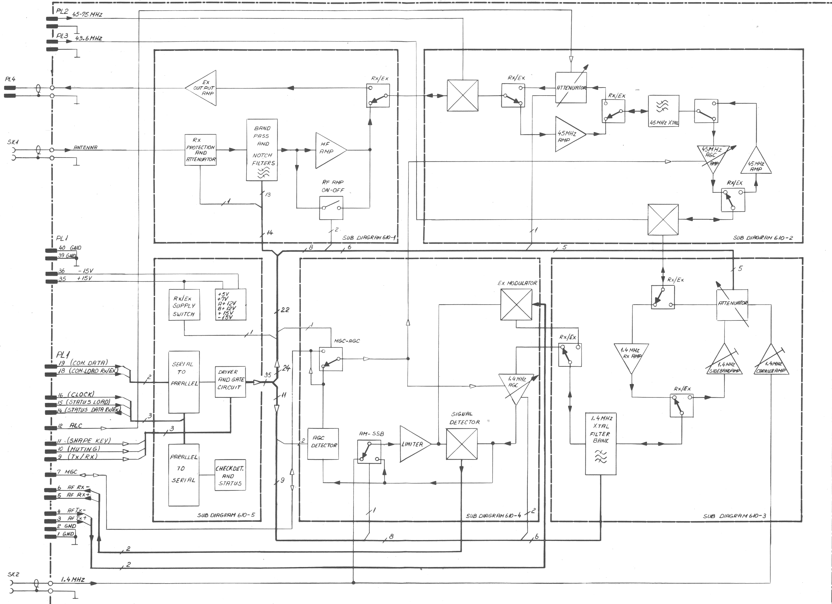
610 MAIN DIAGRAM Rx/Ex SIGNAL PATH VERSION 3A
