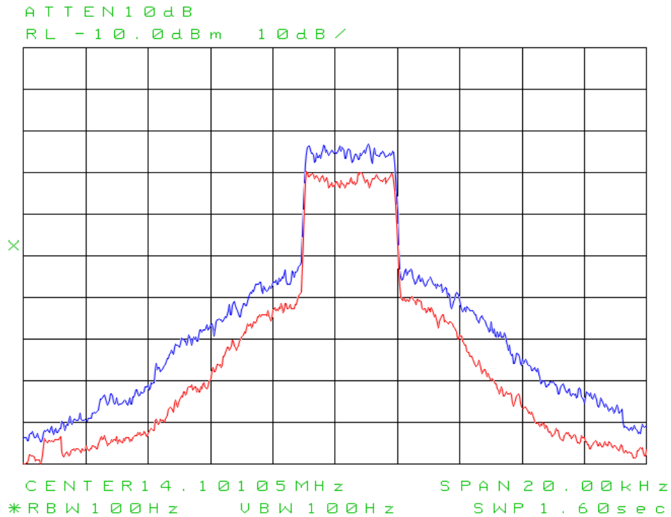
Figure 17: 20m noise modulation, showing IMD skirts.
