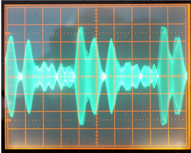
Figure 9: 100W PEP speech envelope, no compression.
