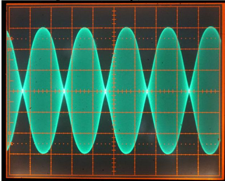
Figure 12: 2-tone envelope, 100W PEP.
