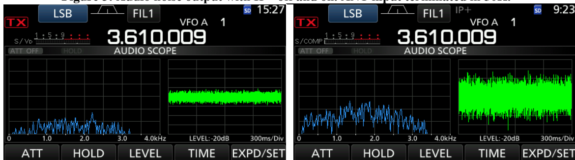
Figure 3: Audio noise output with IP+ off and on. ANT input terminated in 50Ω.
